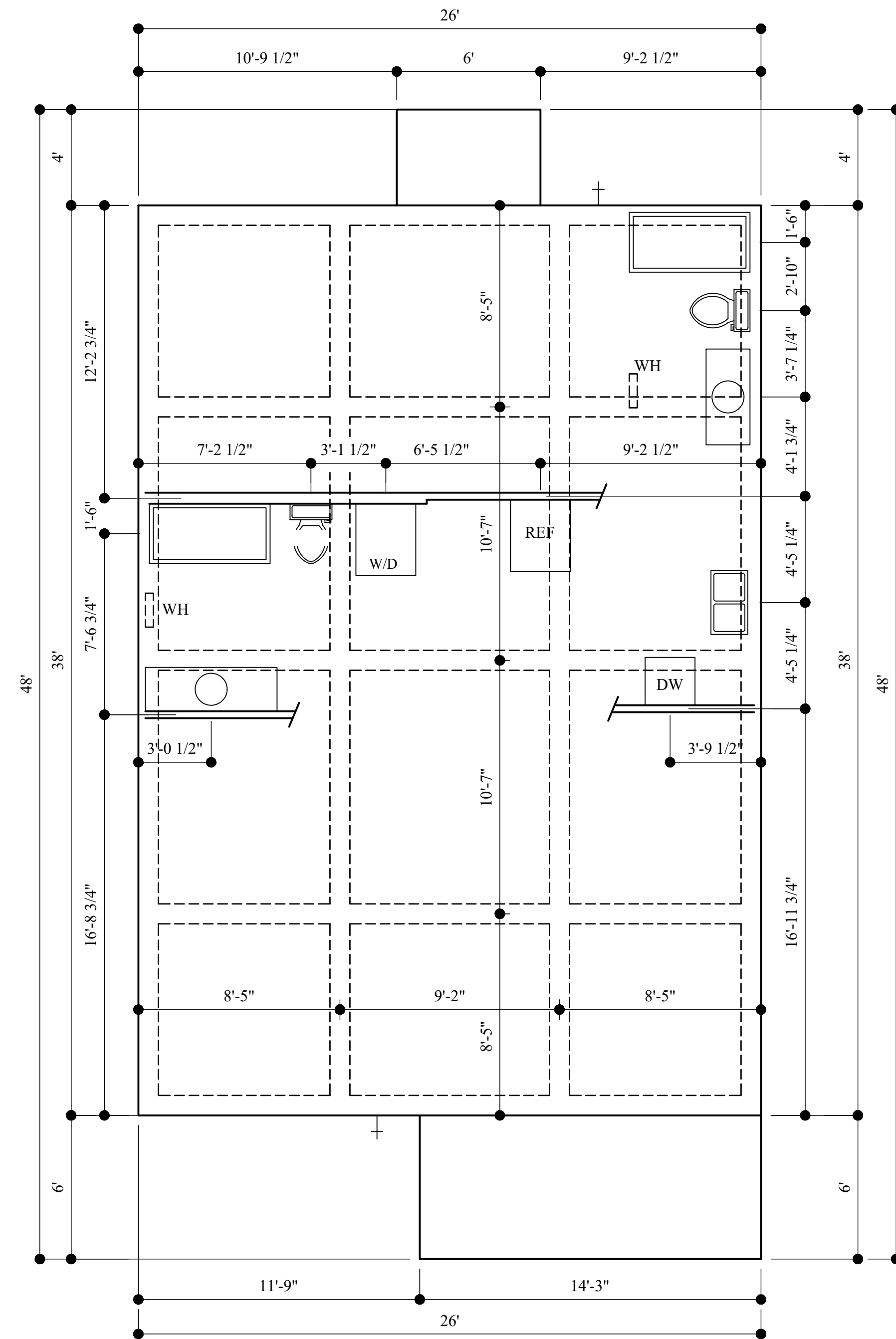
FOUNDATION/ PLUMBING PLAN SCALE 1/4" = 1'-0"
