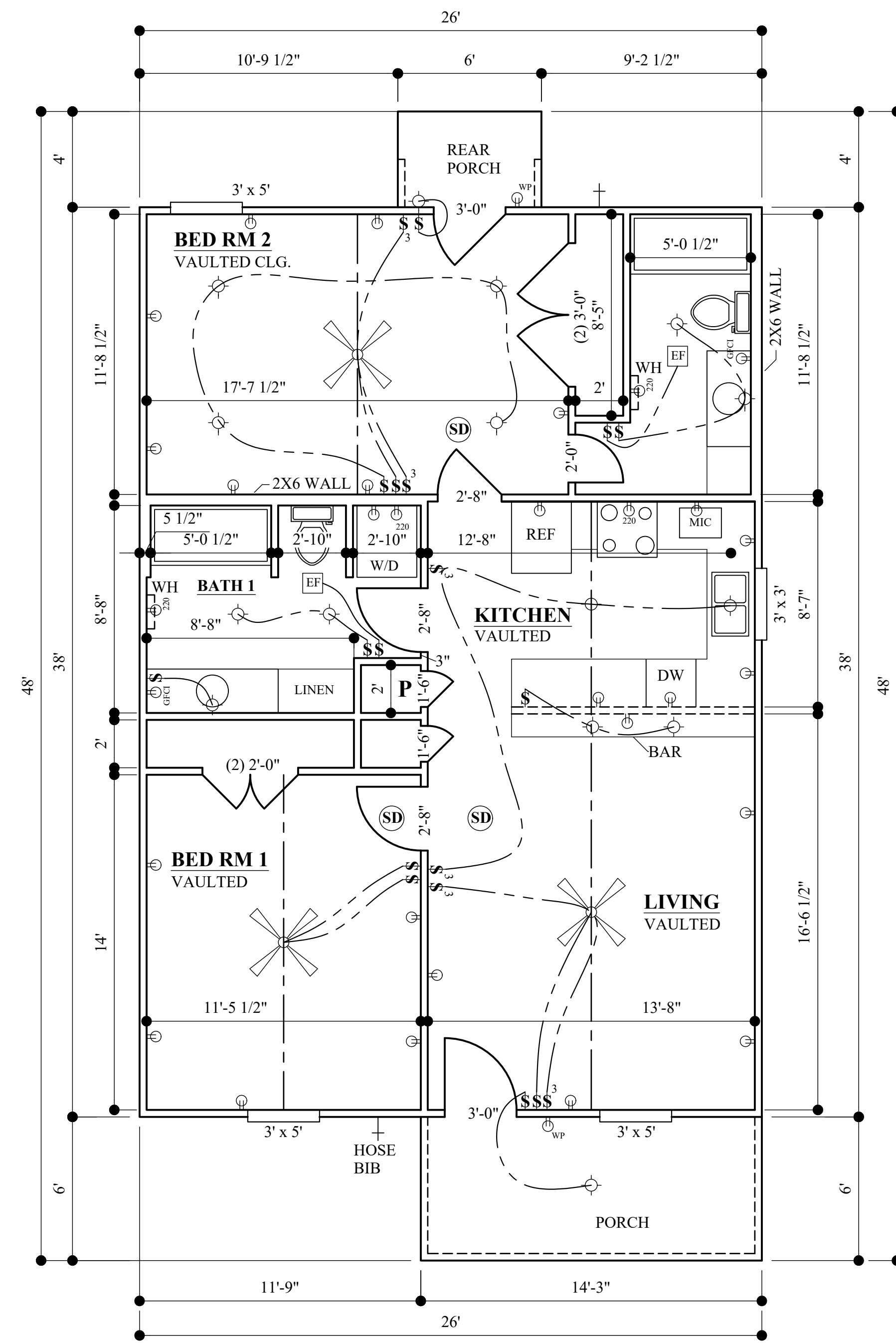
FLOOR PLAN SCALE 1/4" = 1'-0"
