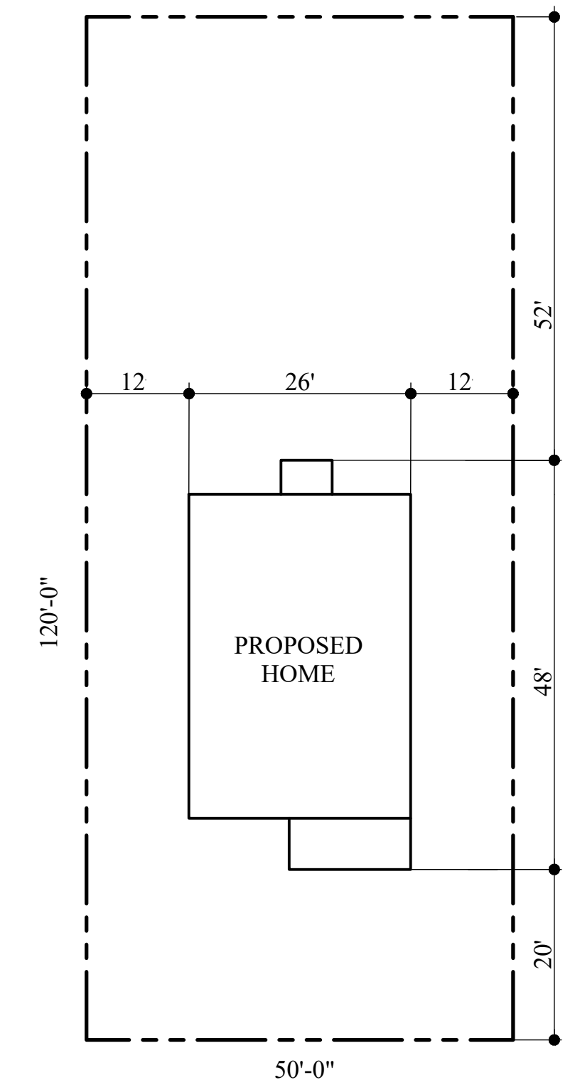
PLOT PLAN SCALE 1/16" = 1'-0"
