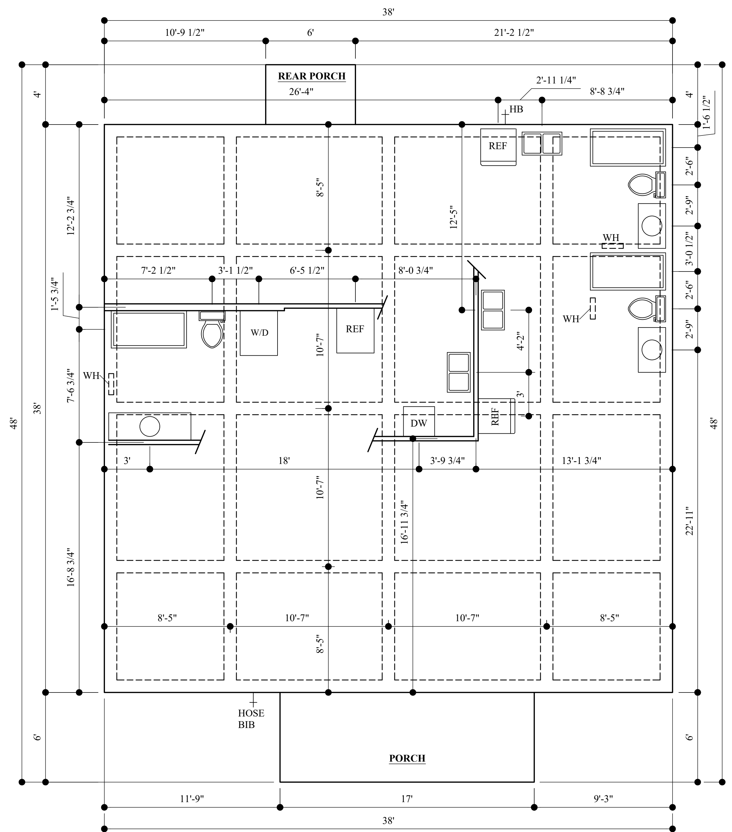
FOUNDATION/ PLUMBING PLAN SCALE 1/4" = 1'-0"
